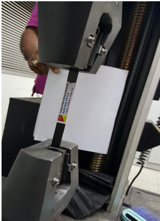
Testing Equipment, Method of Tester Installed, Once Tested the CFRP Cured Laminates Breaking
